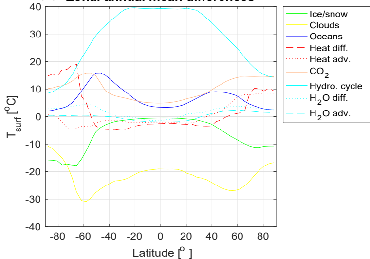
(a) Zonal annual mean differences
