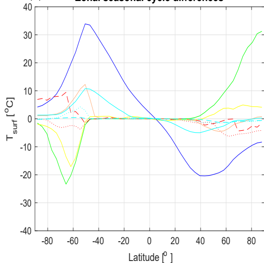
(b) Zonal seasonal cycle differences
