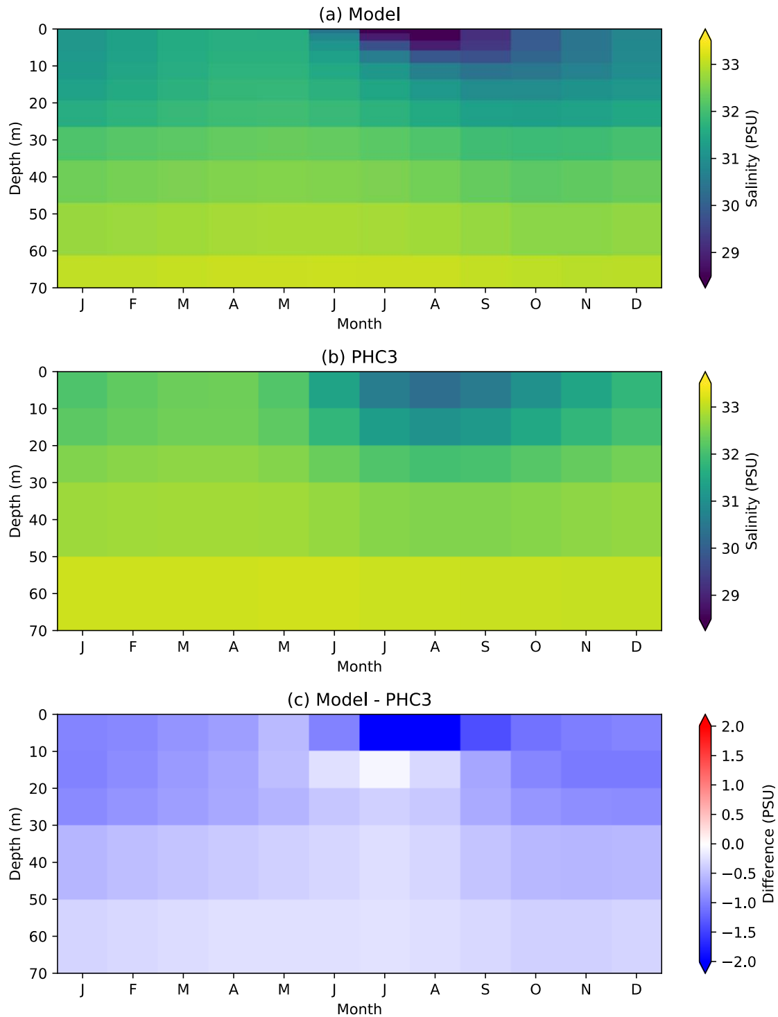
Figure S1: Vertical distribution of salinity in the upper 70-m water column averaged monthly and over the pan-Arctic (north of 66.5N). a) the model output for 1979, b) the Polar Hydrographic Climatology version 3.0, and c) the difference between the two products.
