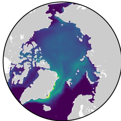
(c) nn_fsbc = 10
