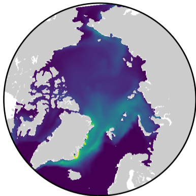
(b) nn_fsbc = 5
