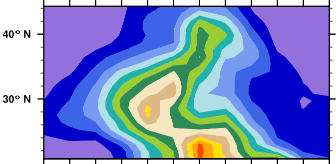
(c) BCC-CSM1.1m
