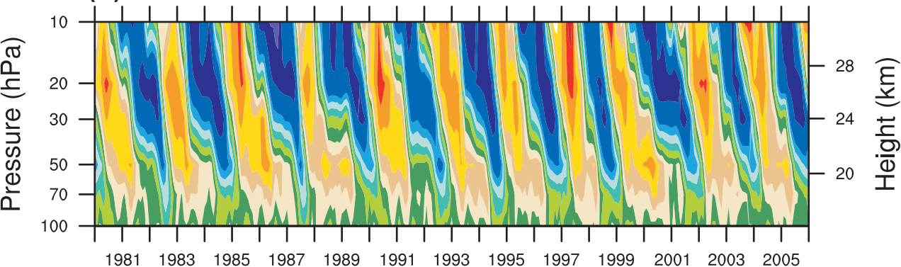
(b) BCC-CSM2-MR
