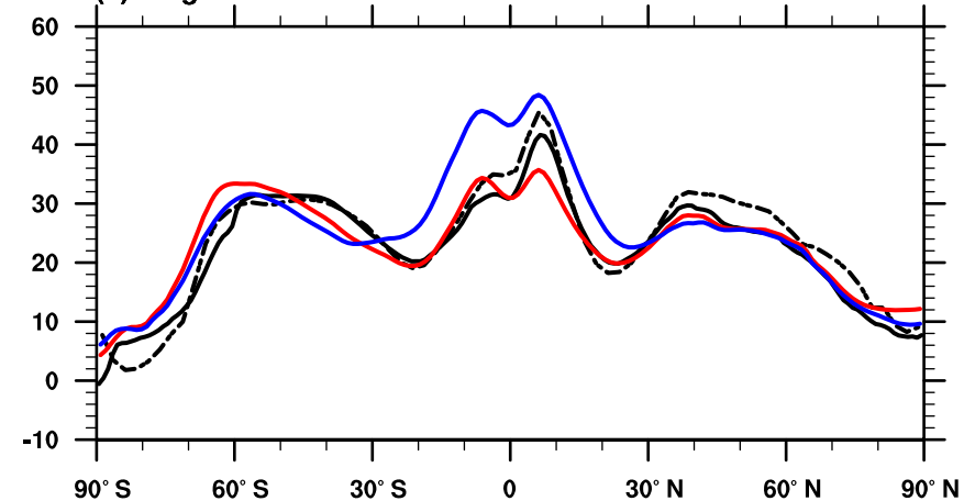
(c) Net CRF
