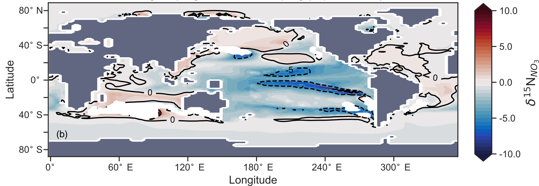
Strong coupling minus weak coupling (euphotic zone)
