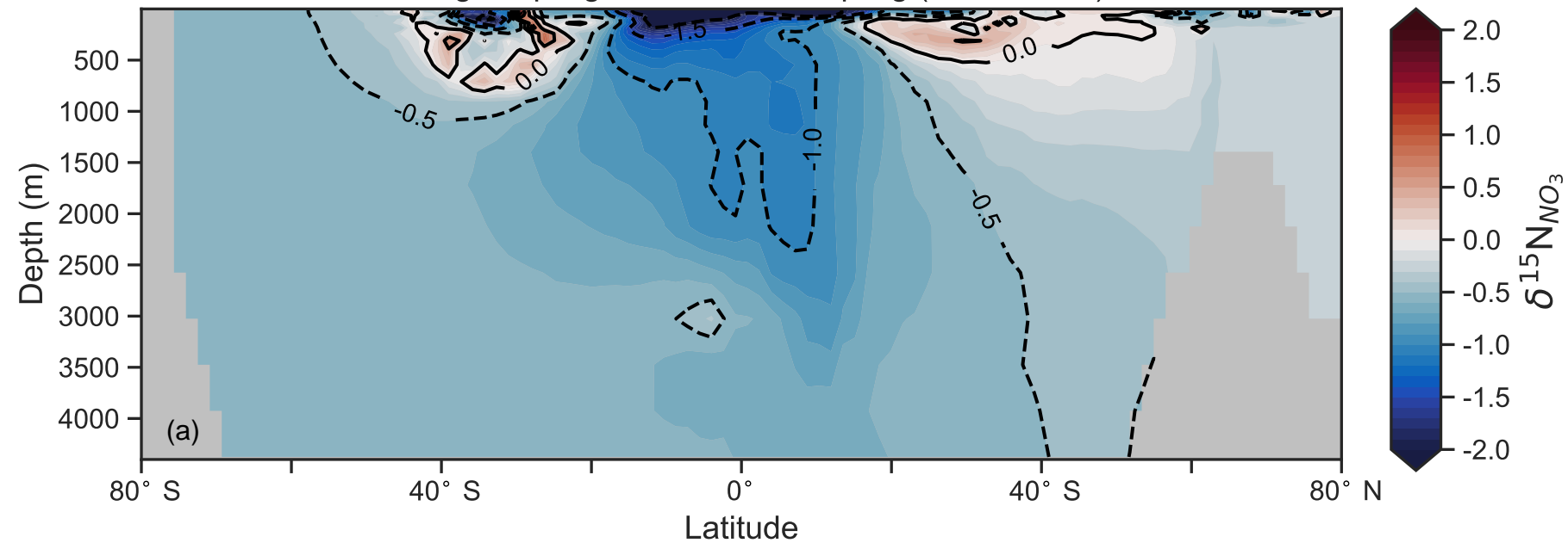
Strong coupling minus weak coupling (zonal mean)
