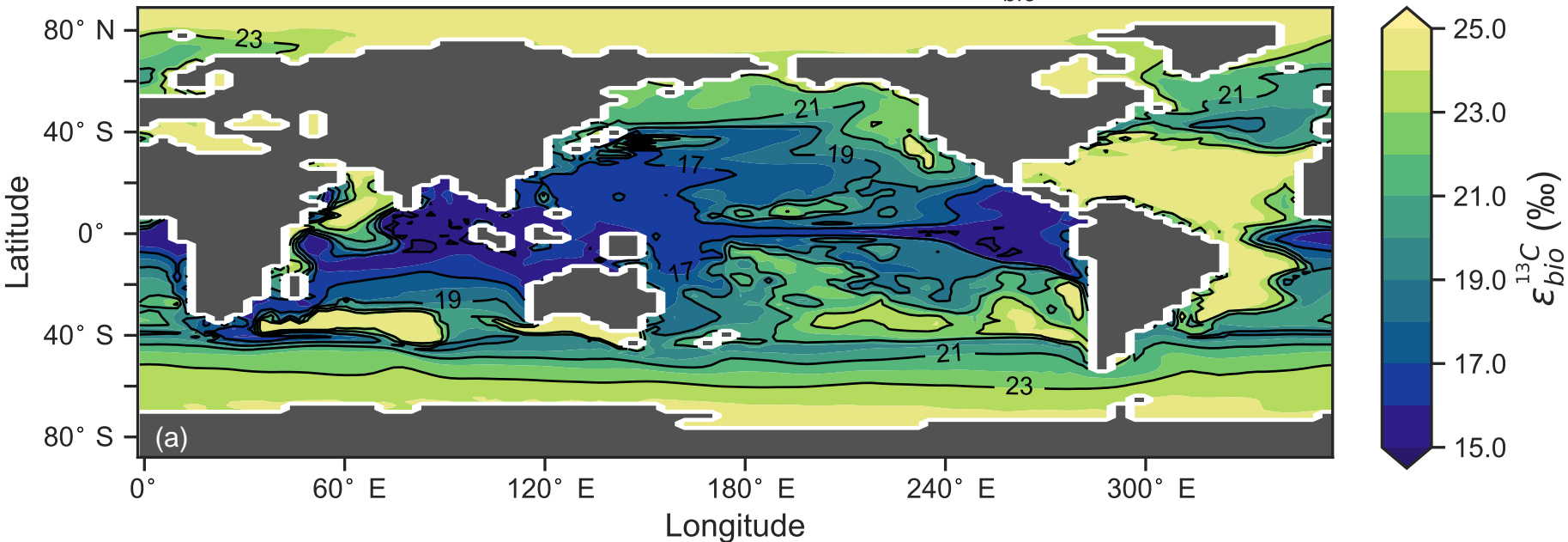
Variable biological carbon fractionation ( \epsilon_{bio}^{13C} )
