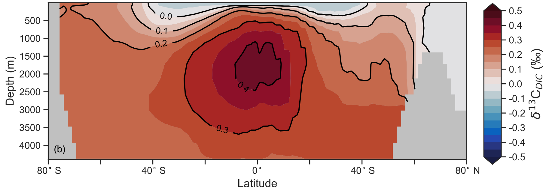
Variable minus static fractionation during biological assimilation
