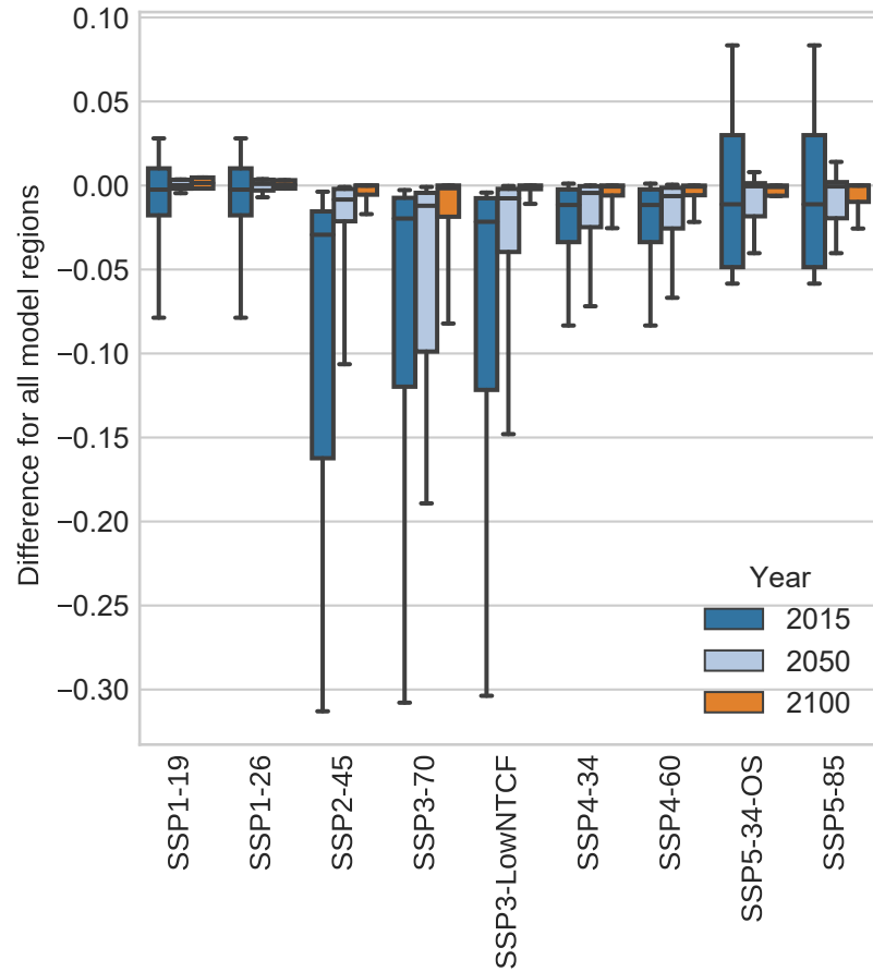
Residential commercial other BC
