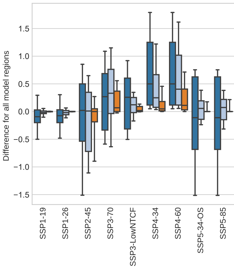
Industrial sector sulfur
