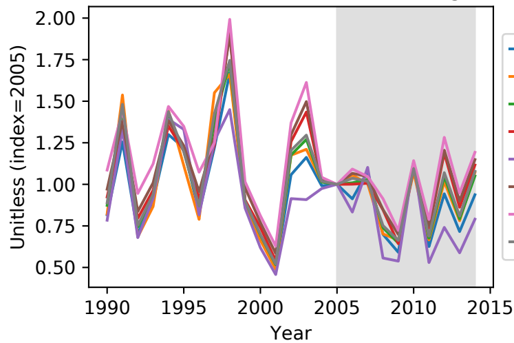
Global emissions peat burning
