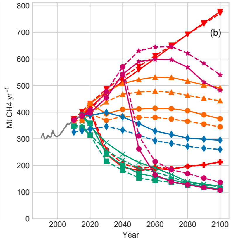
Global CH 4 emissions
