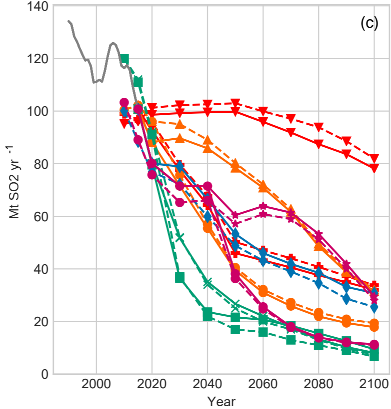
Global sulfur emissions
