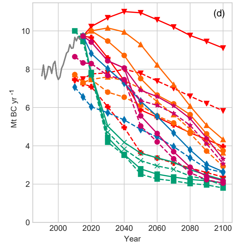
Global BC emissions
