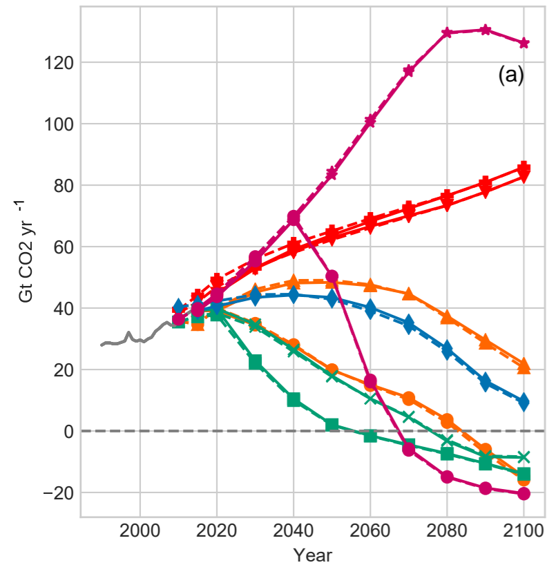
Global CO 2 emissions
