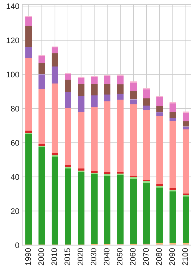
SSP3-7.0 sulfur
