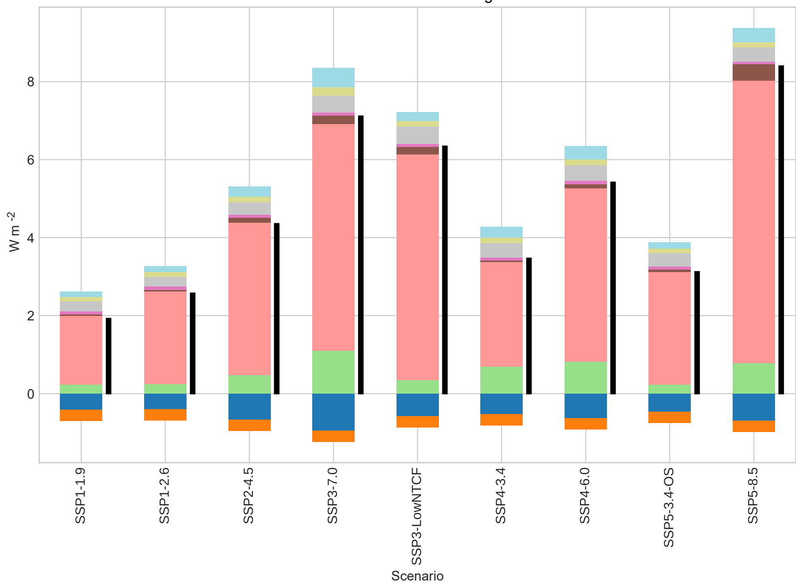
Contribution to radiative forcing in 2100.
