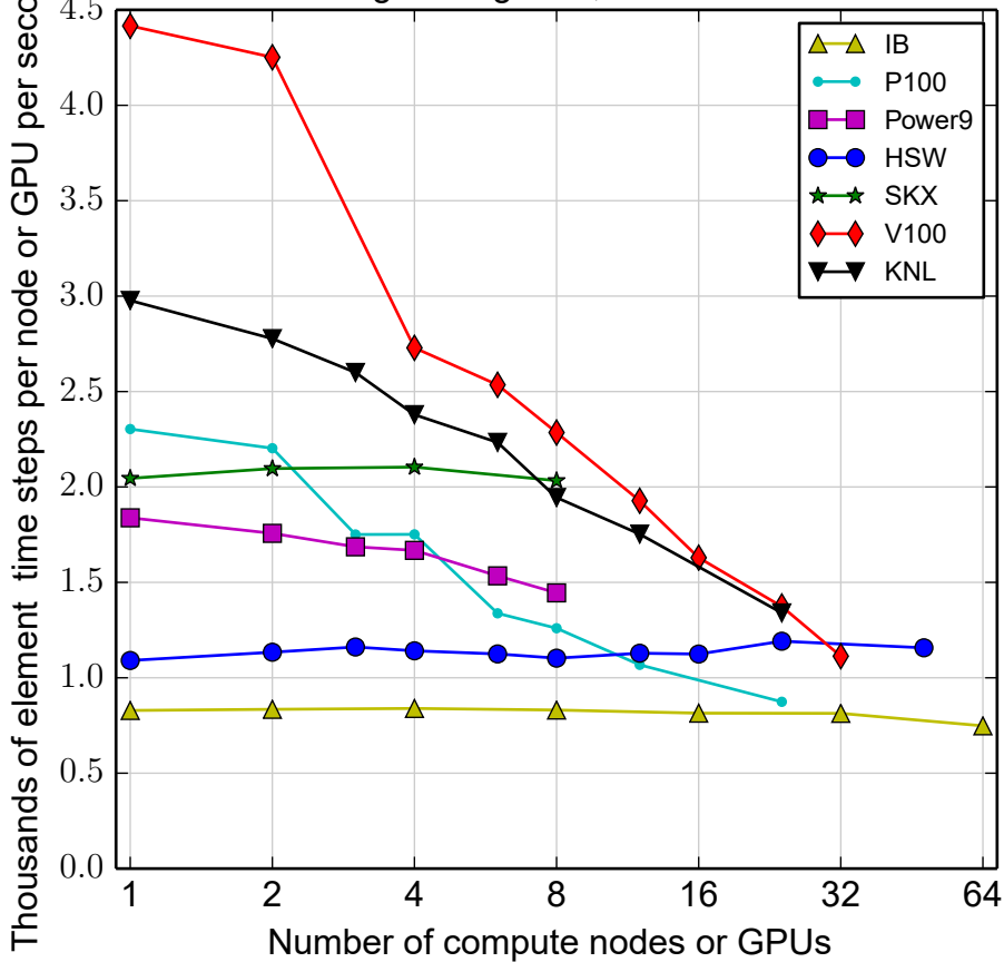
Strong scaling for 1,536 elements
