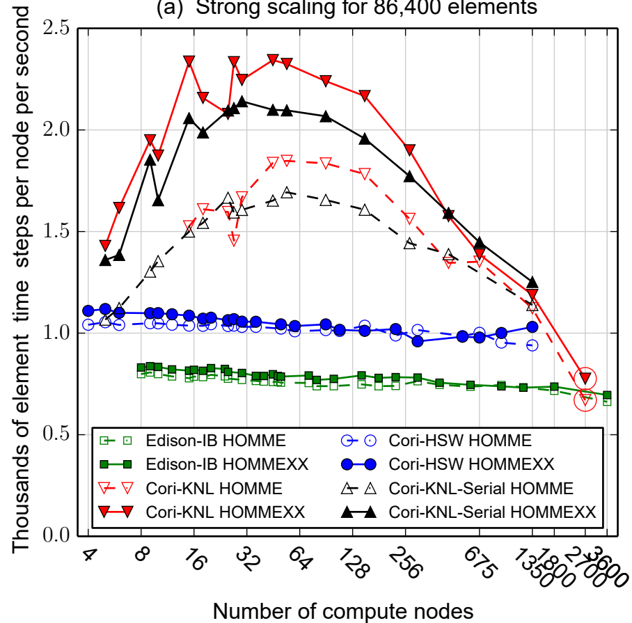
(a) Strong scaling for 86,400 elements
