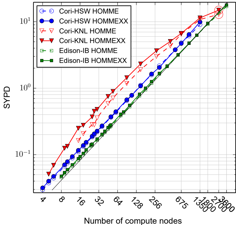
(b) Strong scaling for 86,400 elements
