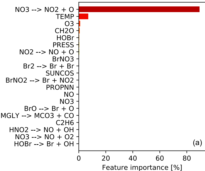
NO:NOx ratio - feature importances
