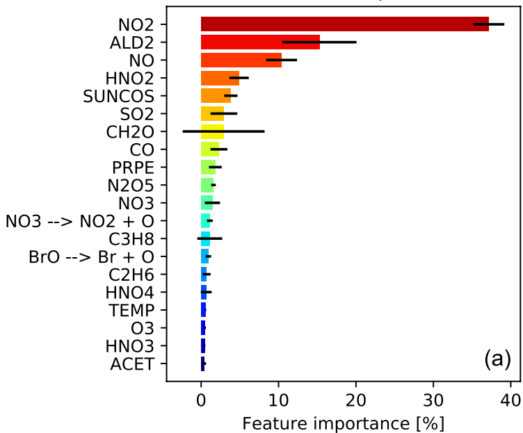
NOx - feature importances
