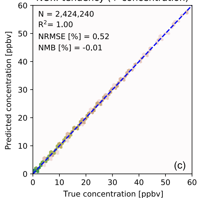
NOx: tendency (+ concentration)
