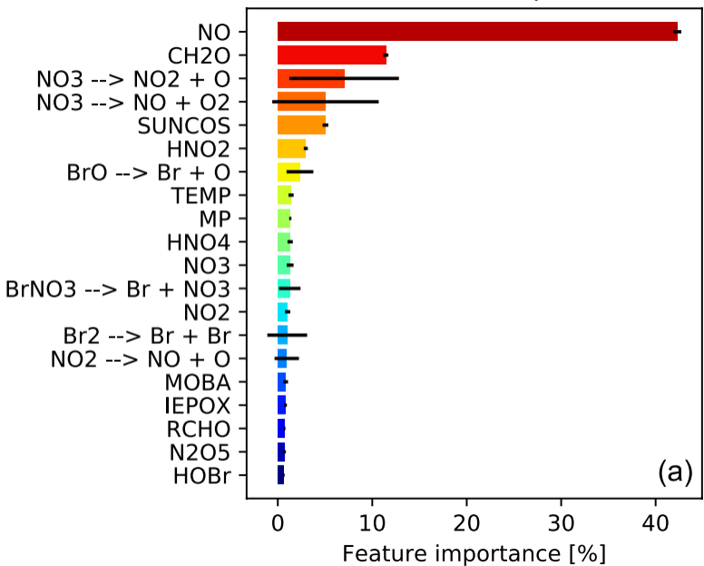
Ozone - feature importances
