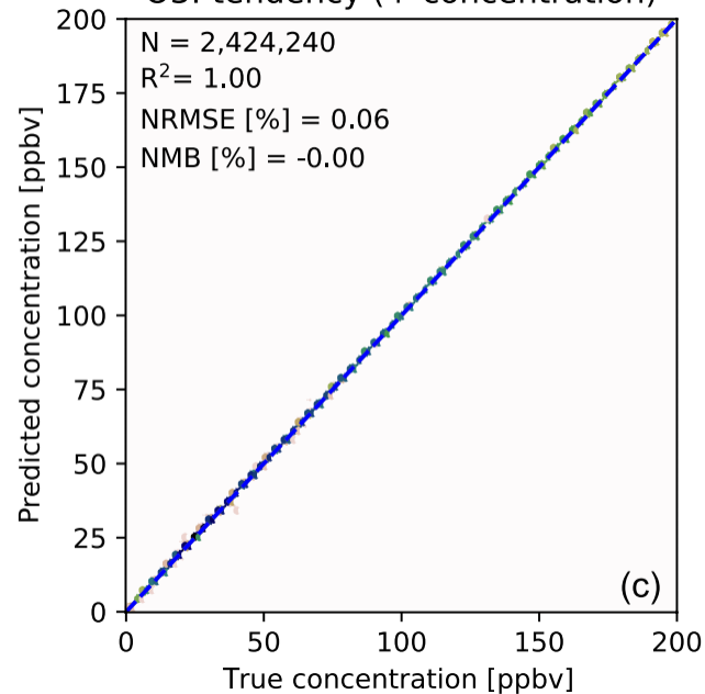
O3: tendency (+ concentration)
