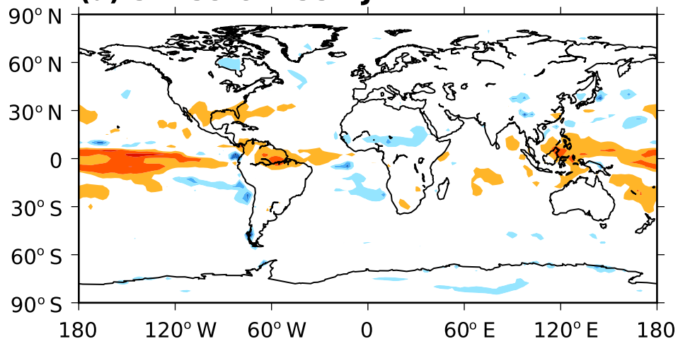
(a) SEAS5 CRPSS DJF
