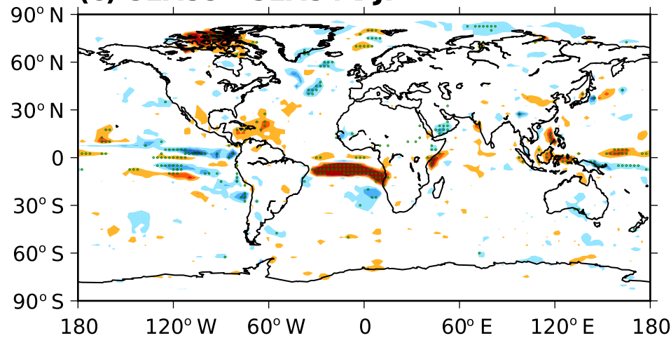
(c) SEAS5 - SEAS4 DJF
