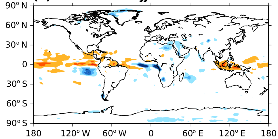
(b) SEAS5 CRPSS JJA
