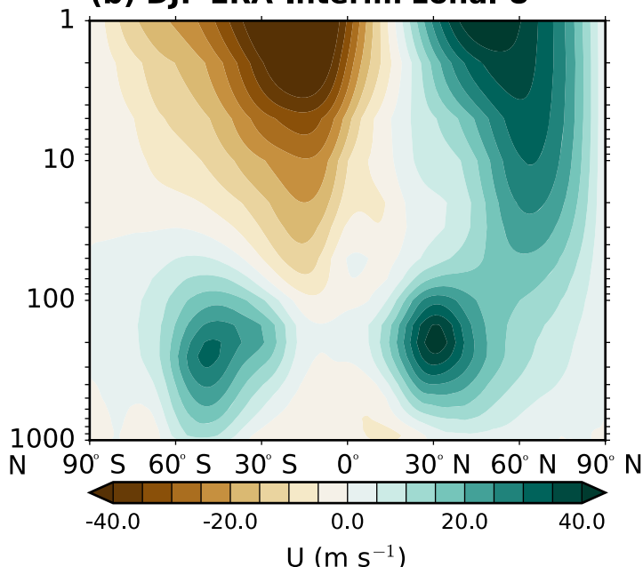
(b) DJF ERA-Interim zonal U
