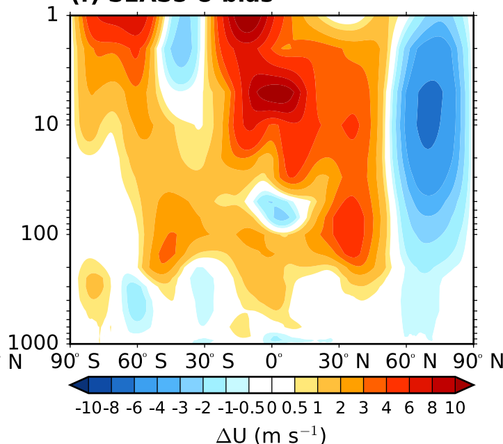
(f) SEAS5 U bias
