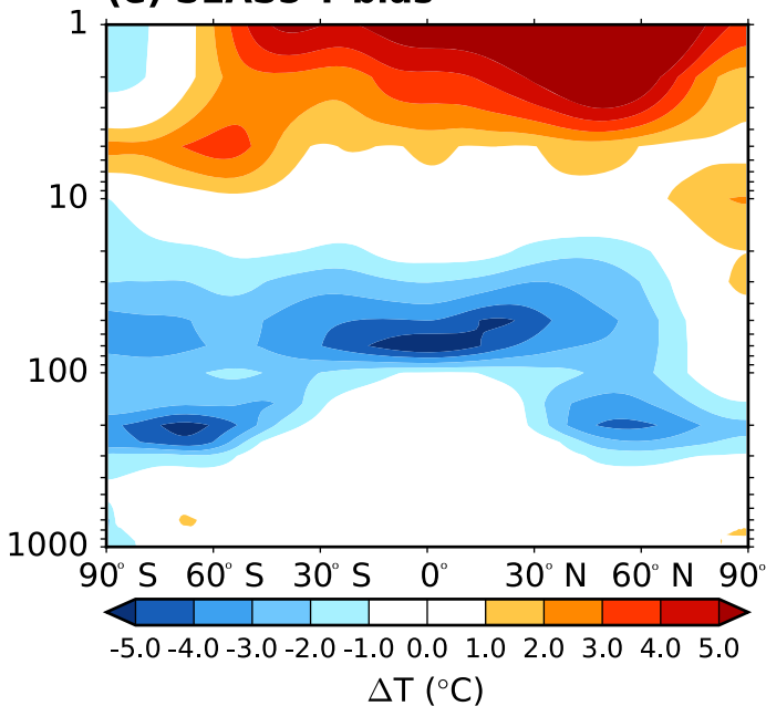
(e) SEAS5 T bias
