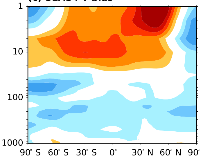
(c) SEAS4 T bias
