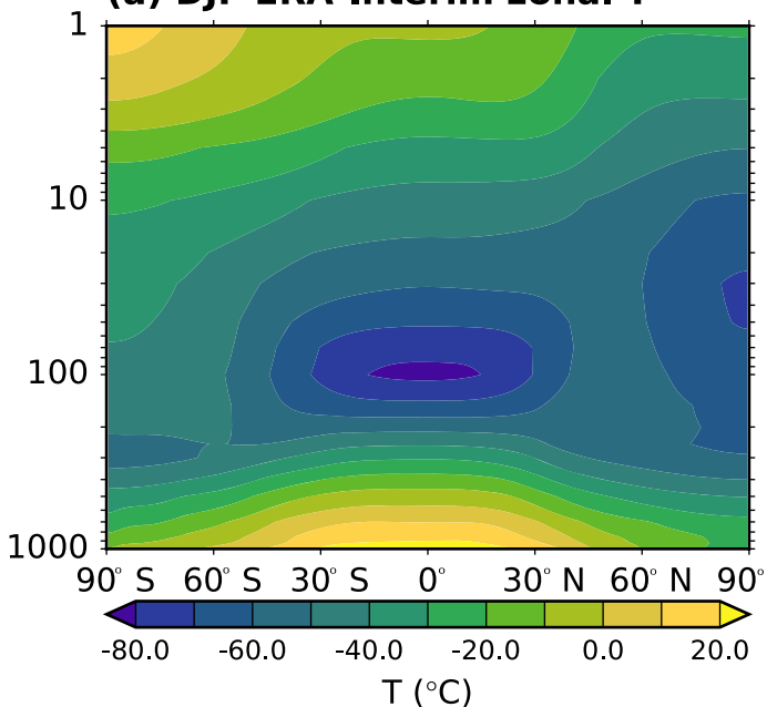
(a) DJF ERA-Interim zonal T
