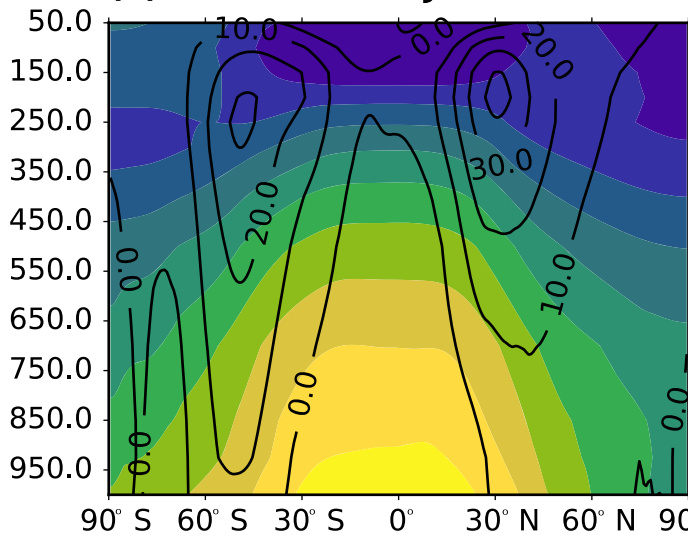
(a) ERA-Interim DJF
