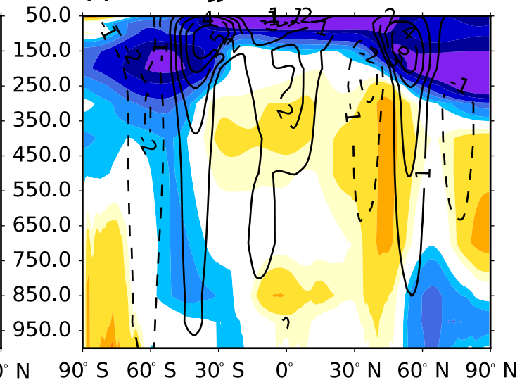
(f) SEAS5 JJA bias
