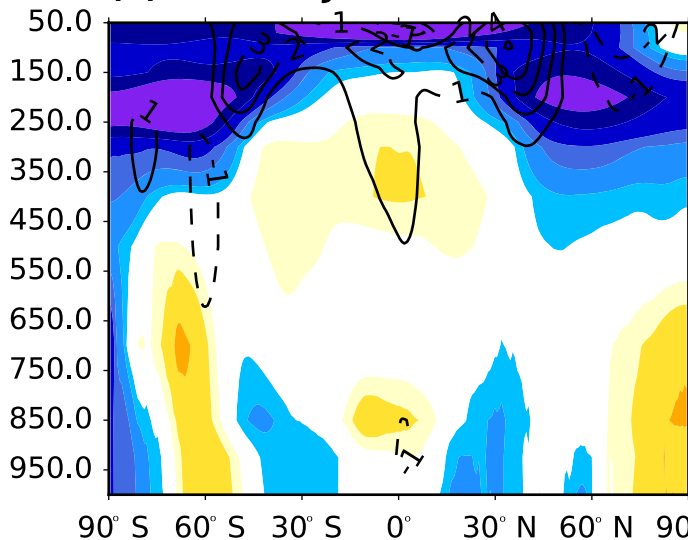
(e) SEAS5 DJF bias
