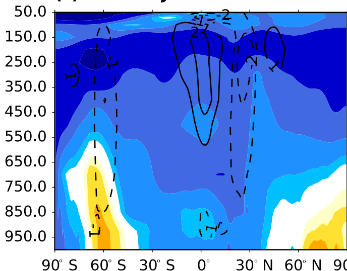
(c) SEAS4 DJF bias
