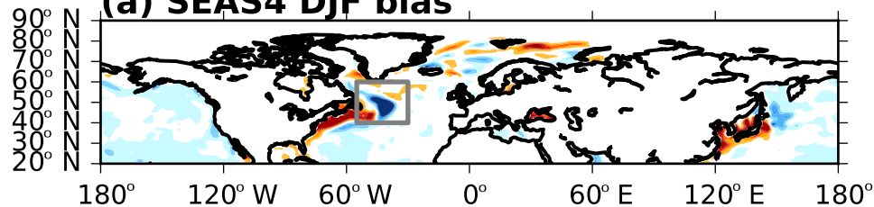
(a) SEAS4 DJF bias
