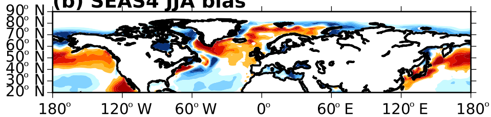
(b) SEAS4 JJA bias
