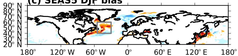
(c) SEAS5 DJF bias
