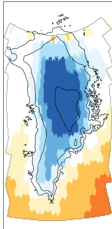
(c) CLOUDSAT
