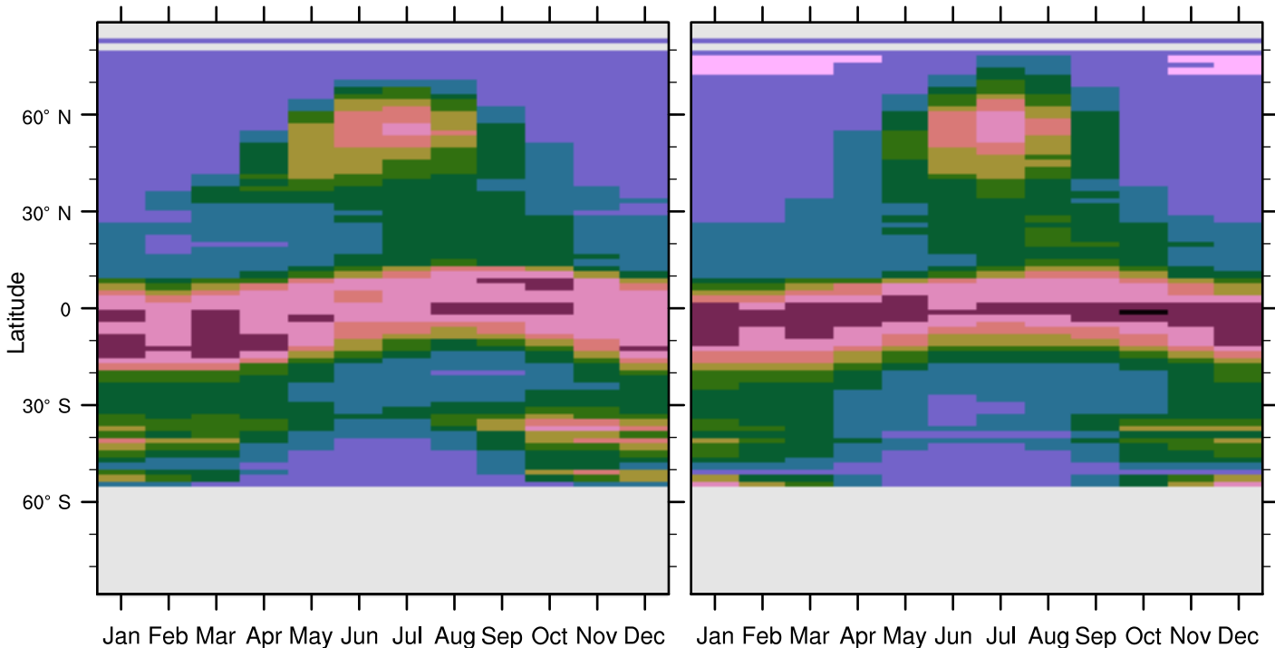
Monthly mean GPP for SEDGES
