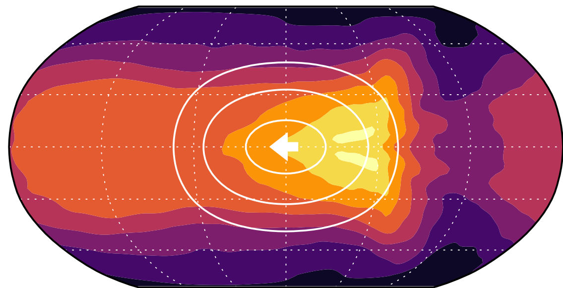
Non-tidally locked
