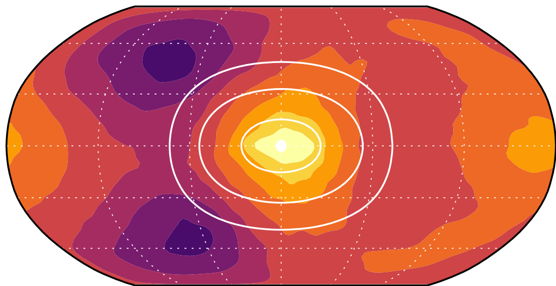
Tidally locked
