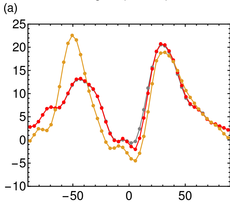
Climatological (500 mb)
