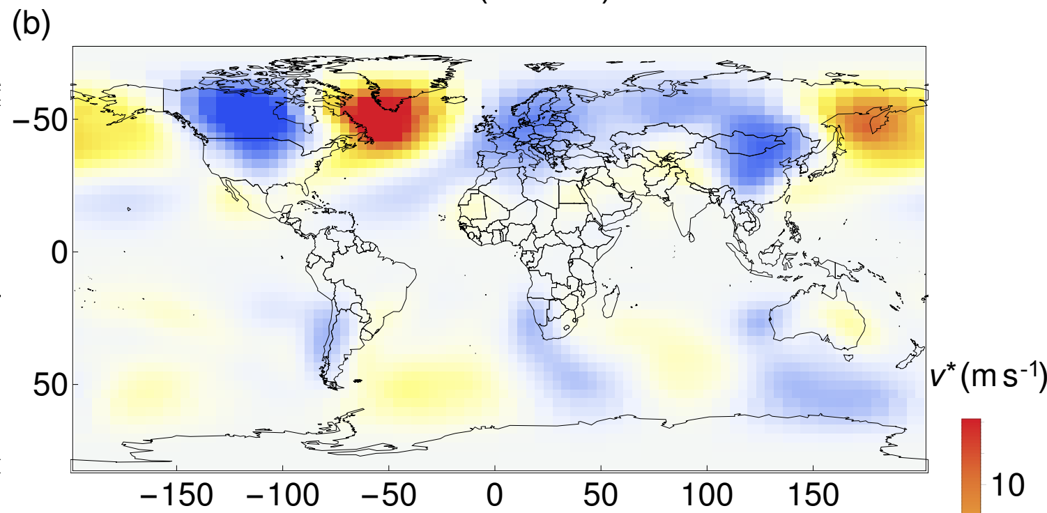
Aeolus v^* (500 mb)
