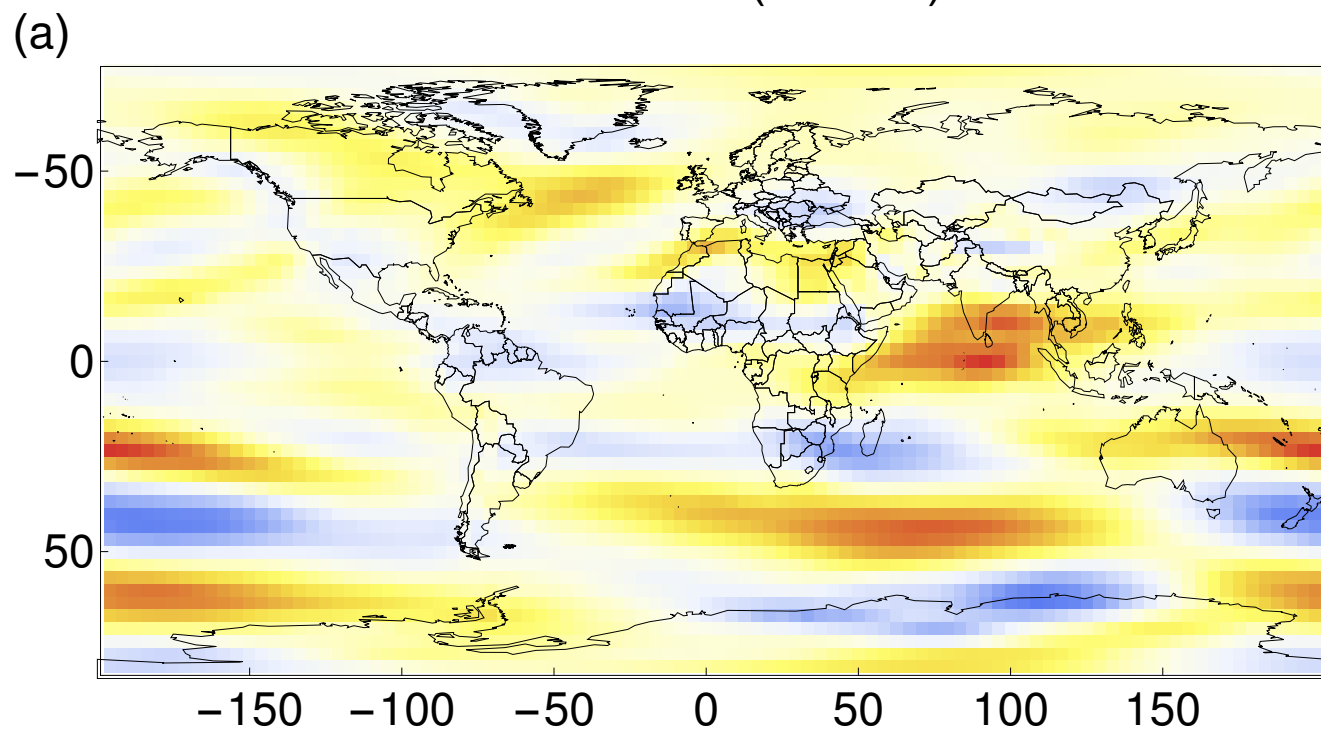
ERA-Interim u^* (500 mb)
