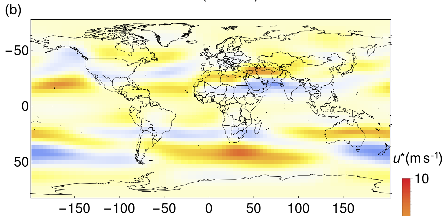
Aeolus u^* (500 mb)
