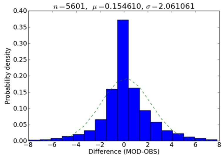
(c) BEPS
