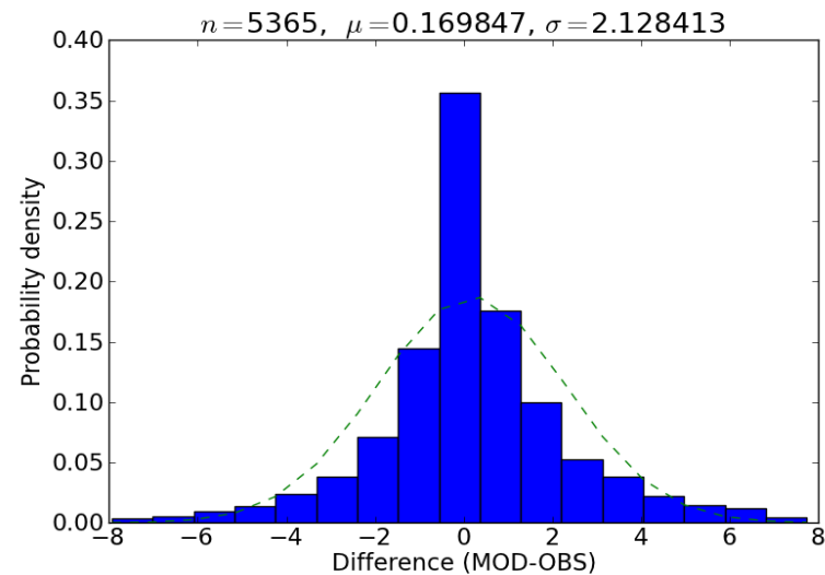
(a) CTEM-CRUNCEP
