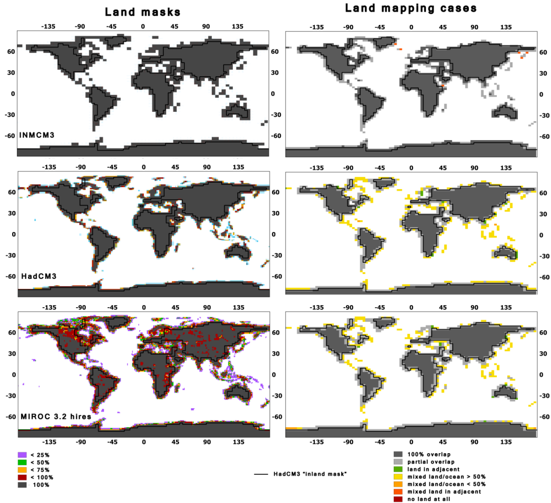
Figure S2. Three examples of GCM grids (on the left), representing main grid categories in the CMIP3 dataset. Diagrams on the right show where different re-gridding strategies were applied in order to translate each grid-box into the UKMO-HadCM3 GCM land grid-boxes.
