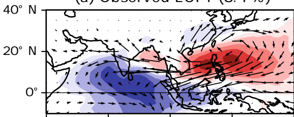
(a) Observed EOF1 (8.4 %)
