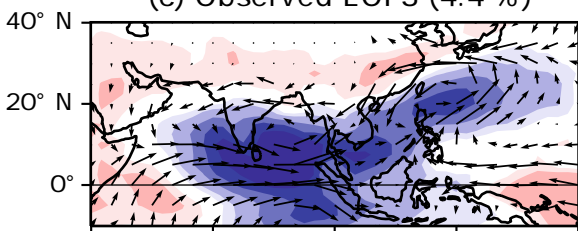
(c) Observed EOF3 (4.4 %)
