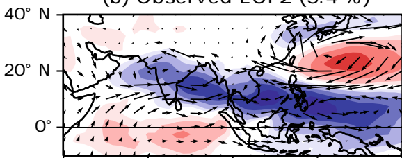
(b) Observed EOF2 (5.4 %)
