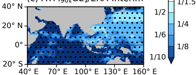
(c) \text{ATM}_{90}[\tilde{G}\tilde{L}]/\text{ERA-Interim}
