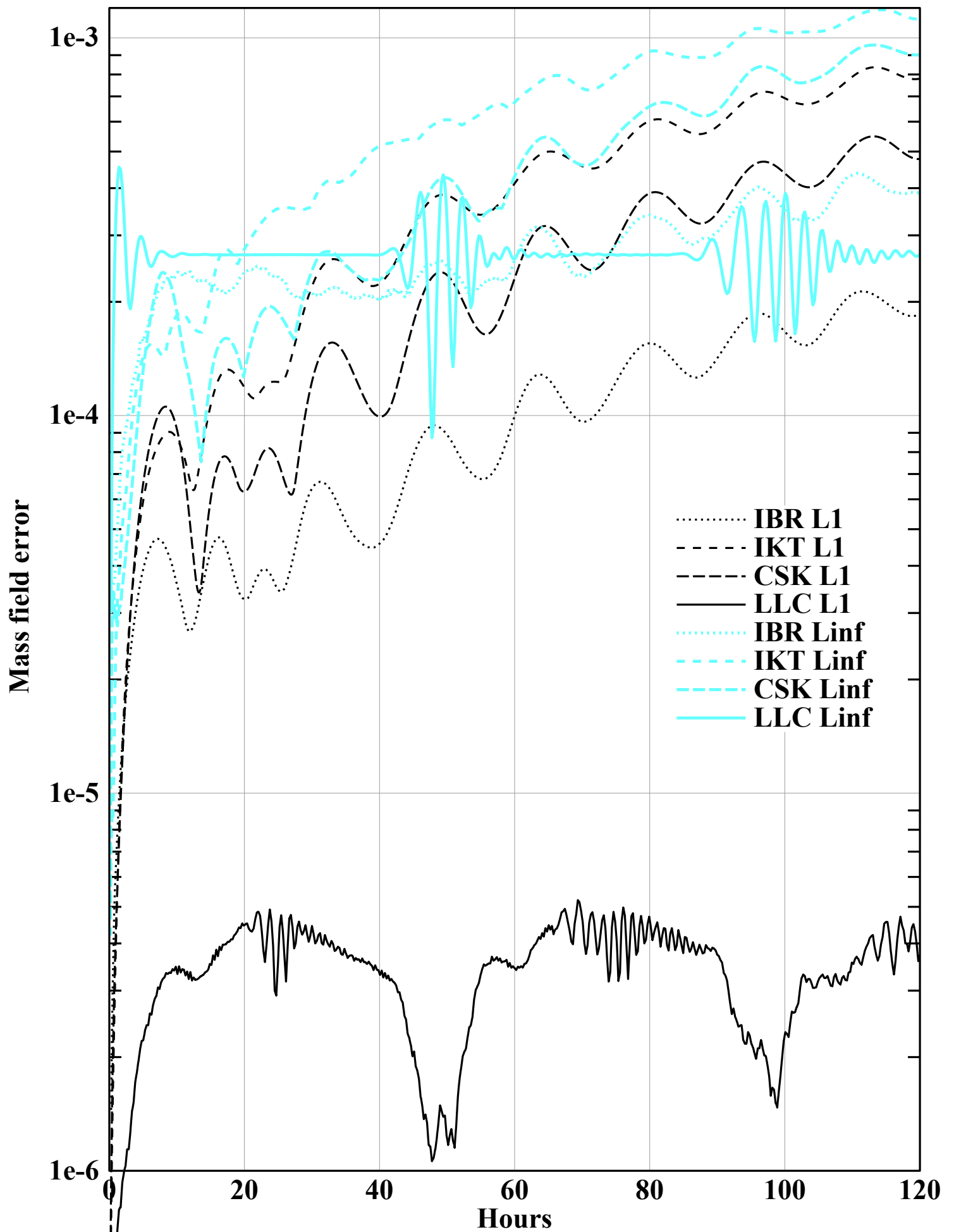
Mass field error for L1 and Linfinity norms
