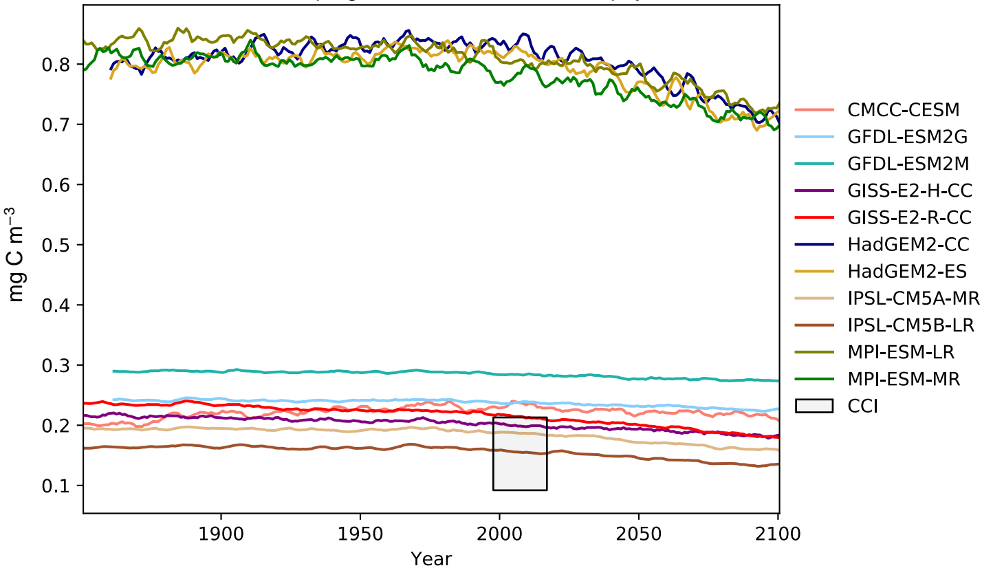
RCP 8.5 r1i1p1 global surface mean chlorophyll
