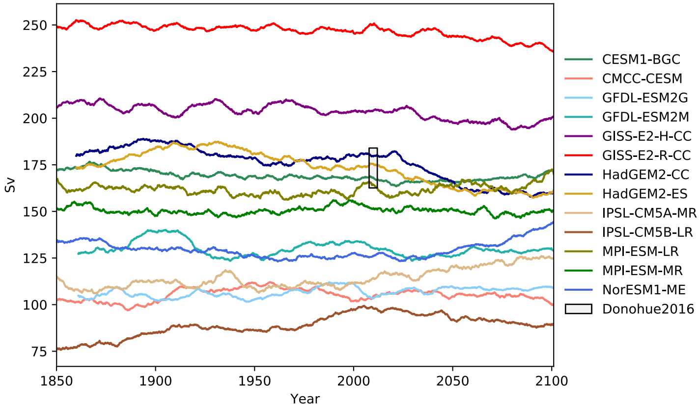
RCP 8.5 r1i1p1 Drake Passage transport
