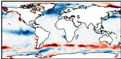
(c) Difference
