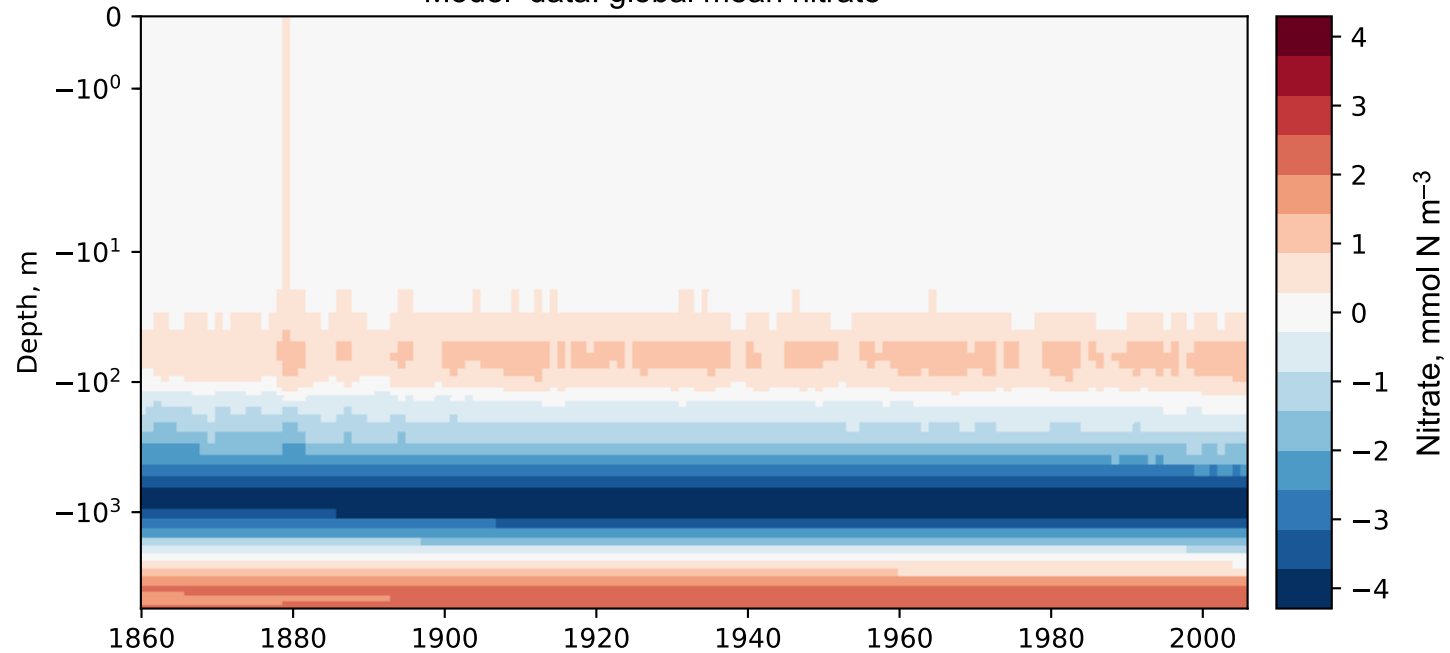
Model–data: global mean nitrate
