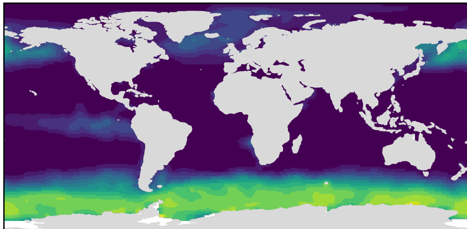
(b) WOA surface nitrate
