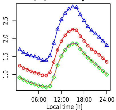
H 2 O 2 diurnal cycle
