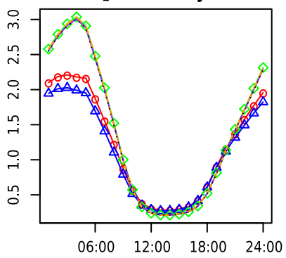
NO 2 diurnal cycle
