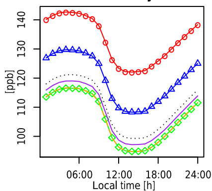
CO diurnal cycle
