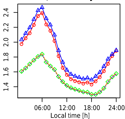
SO 4 -2 diurnal cycle
