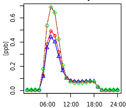
NO diurnal cycle
