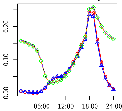
SO 4 -2 diurnal cycle
