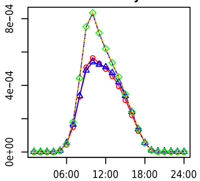
OH diurnal cycle
