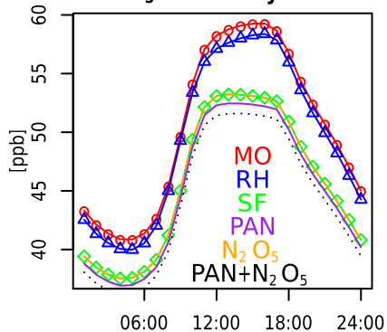
O 3 diurnal cycle
