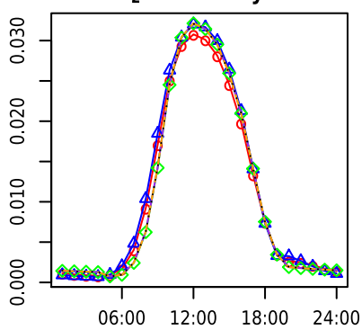
HO 2 diurnal cycle
