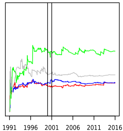
(b) Northeastern US
