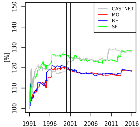
(a) Midwestern US
