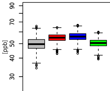
(b) Western US
