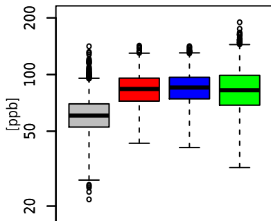
(g) 1x1 Midwestern US
