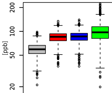
(h) 1x1 Northeastern US
