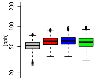
(f) Southeastern US
