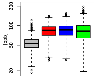
(i) 1x1 Southeastern US
