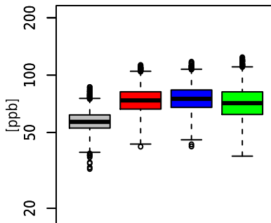
(e) Northeastern US
