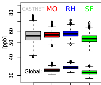
(a) Continental US
