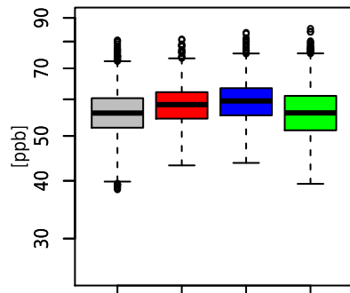
(c) Eastern US
