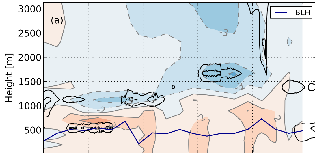
(a) and (c): T [ ^{\circ}C ]
