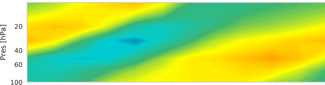
ICON-ART feedback
