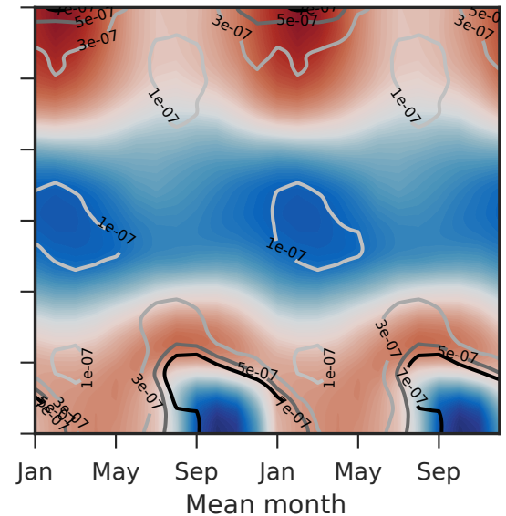
(c) ICON-ART feedback
