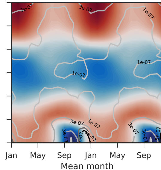
(b) ICON-ART ctrl Linoz
