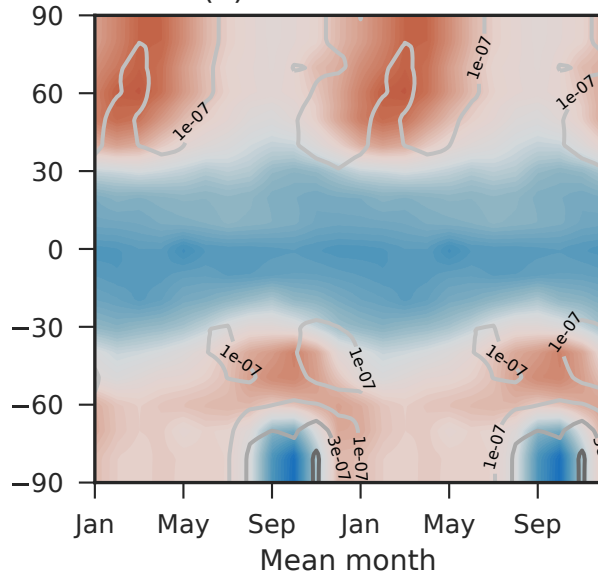
(a) ICON-ART ctrl
