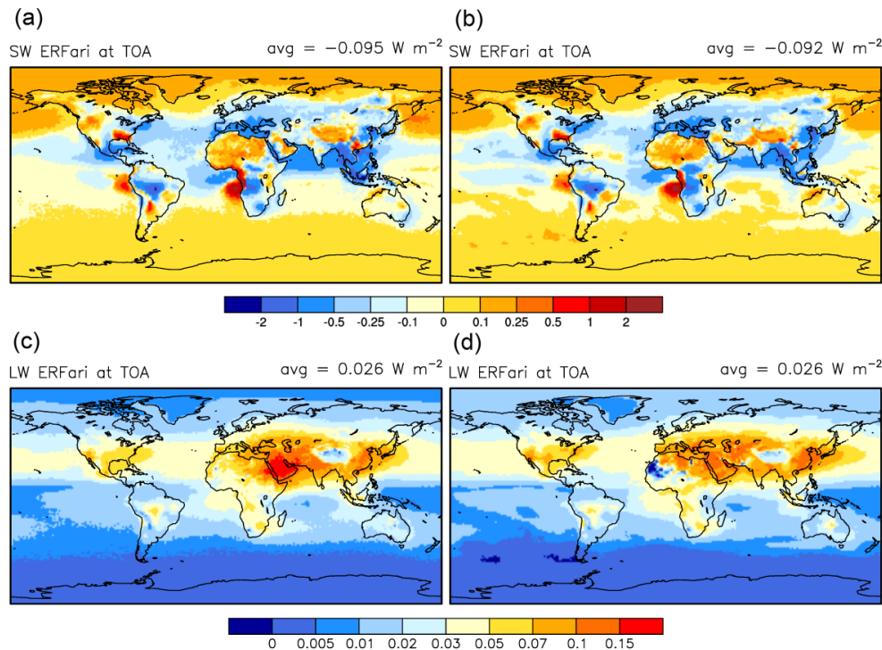
Figure 9. Shortwave (SW, a and b ) and longwave (LW, c and d ) ERFari at the top of the atmosphere (TOA) for the simulations NUDGE_PD–NUDGE_PI ( a and c ) and AMIP_PD–AMIP_PI ( b and d ). Note the different color scales. Note also that the semi-direct effect is not included here, since ERFari in this study corresponds to the “direct radiative forcing” component in Ghan (2013).
