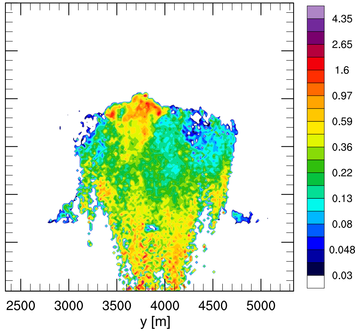
(b) Precip.rate (mm h -1 )
