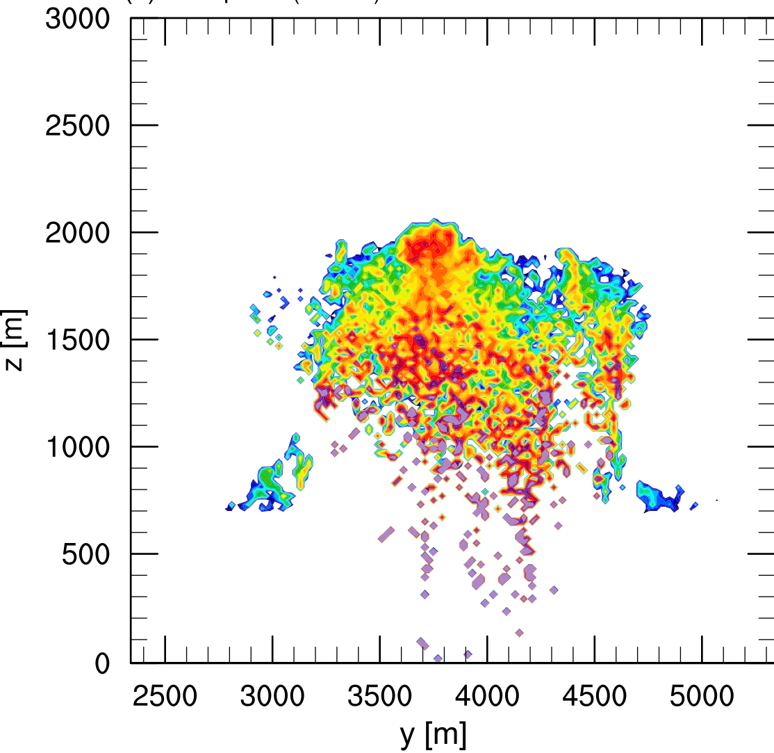
(a) Precip.rate (mm h -1 )
