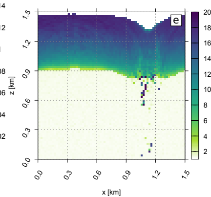
cloud droplet effective radius [ \mu\text{m} ]
