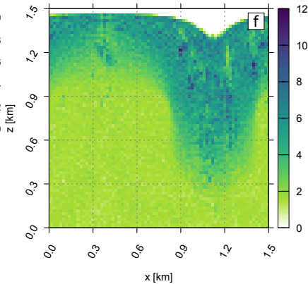
S^{\text{VI}} conc. [mol/ \mu\text{g} of dry air]
