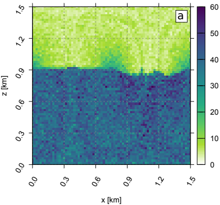
dry radius [ \mu\text{m} ]
