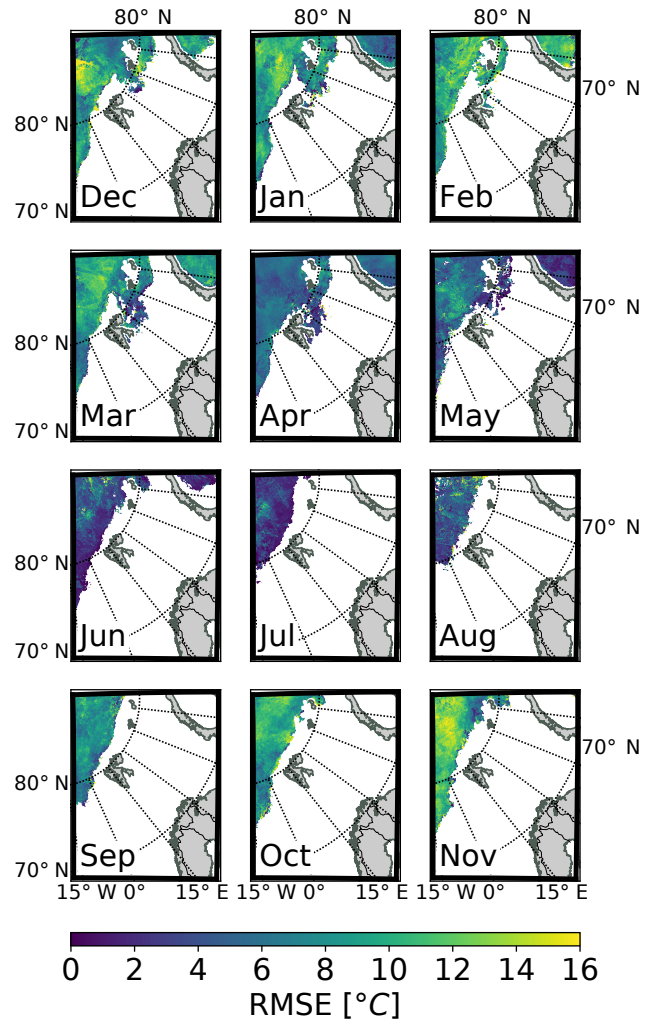
Figure 13. Spatial distribution of the monthly root mean square error (RMSE) of the ice surface temperature after 66 h of AA-PREScribed forecast initialized at 00:00 UTC. Monthly RMSEs are calculated using the MODIS ice surface temperature product and cover the time period from 1 December 2015 to 1 December 2016.
