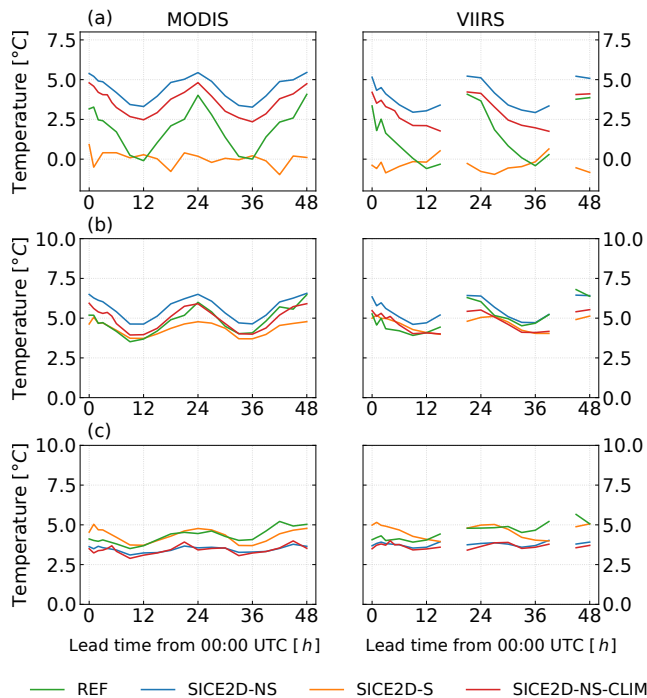
Figure 9. Mean bias, root mean square error, and standard deviation of errors in the ice surface temperature forecasts initialized at 00:00 UTC, calculated using MODIS (left panel) and VIIRS (right panel) ice surface temperature products, as a function of lead time for the period from 1 March to 30 April 2013 for REF, SICE2D-NS, SICE2D-S, and SICE2D-NS-CLIM. (a) Mean bias; (b) root mean square error (RMSE); (c) standard deviation of errors (ESTD). VIIRS swaths for the lead times of 18 and 42 h systematically cover only a minor part of the AROME Arctic domain. They were excluded as not representative.
