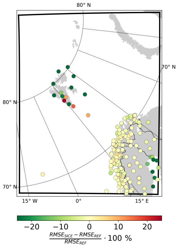
Figure 2. Relative change (in percent) in RMSE of the 2 m temperature forecasts between SICE2D-NS and REF. Negative values mean that the RMSE is smaller in SICE2D-NS than in REF. Forecasts starting at 00:00 UTC within the time period from 1 March to 30 April 2013 were used for comparison.
