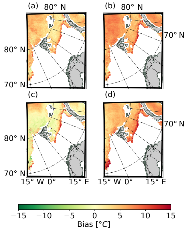
Figure 10. Spatial distribution of the mean error of the ice surface temperature after 24 h of forecast starting at 00:00 UTC for REF, SICE2D-NS, SICE2D-S, and SICE2D-NS-CLIM compared to the MODIS product. Mean errors are calculated for the time period from 1 March to 30 April 2013. (a) REF; (b) SICE2D-NS; (c) SICE2D-S; (d) SICE2D-NS-CLIM.
