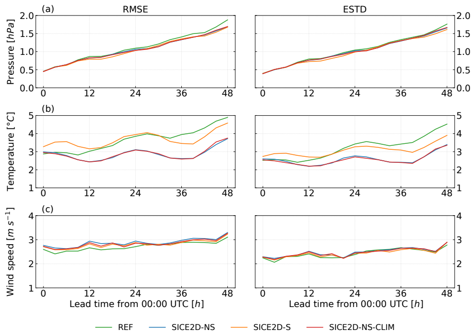
Figure 4. Root mean square error (RMSE, left panels) and standard deviation of errors (ESTD, right panels) as a function of lead time for forecasts initialized at 00:00 UTC for experiments REF, SICE2D-NS, SICE2D-S, and SICE2D-NS-CLIM over the AROME Arctic domain for the period from 1 March to 30 April 2013. Series are calculated for seven Svalbard stations. (a) Mean sea level pressure; (b) 2 m temperature; (c) 10 m wind speed.
