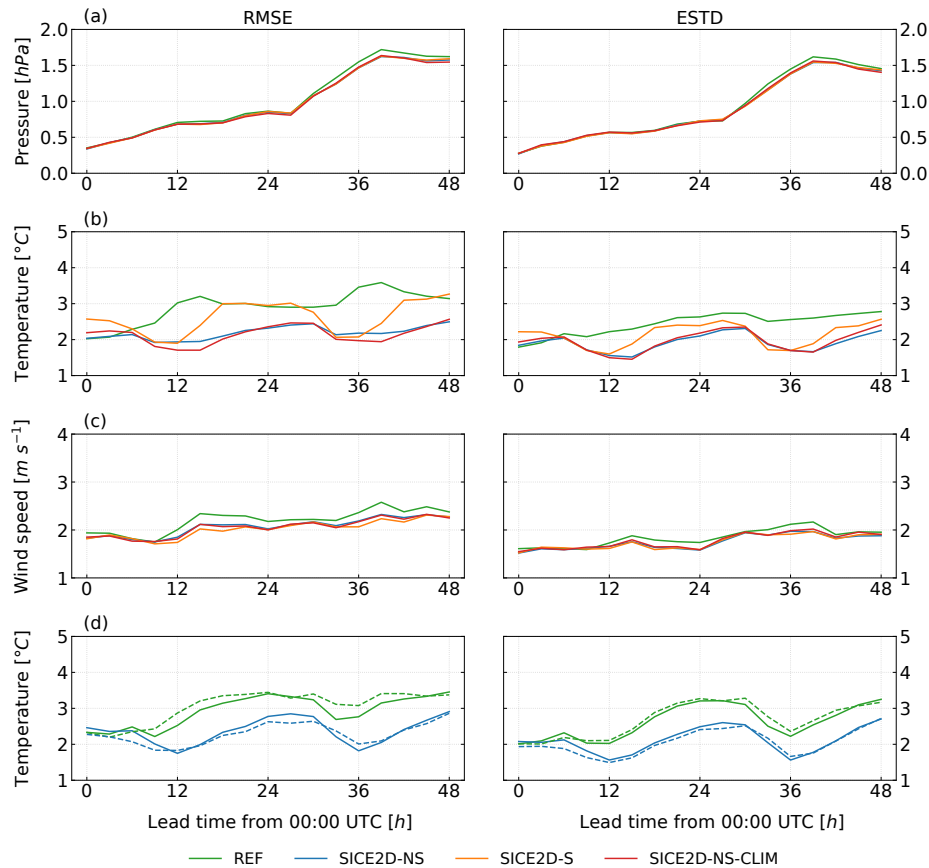
Figure 5. Same as Fig. 4, but for seven stations located in the coastal area of the Gulf of Bothnia. Panel (d) shows the same error statistics as panel (b) but only for March 2013 for experiments REF and SICE2D-NS over the AROME Arctic (solid lines) and MetCoOp (dashed lines) domains.
