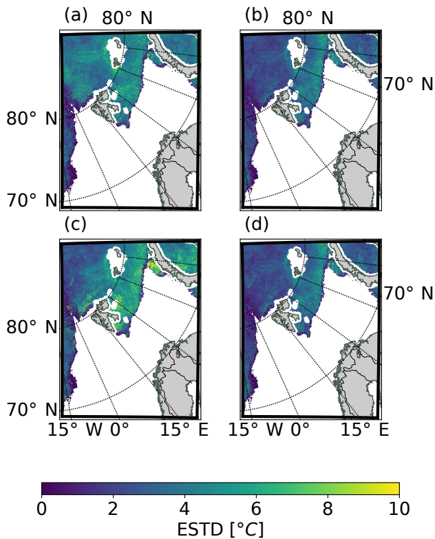
Figure 11. Same as Fig. 10, but showing the spatial distribution of the standard deviation of errors (ESTD).
