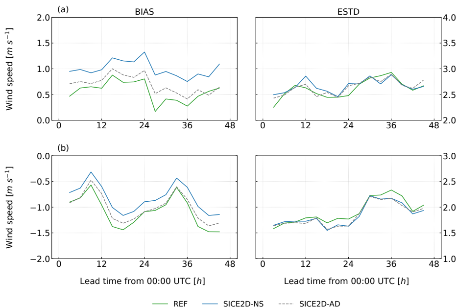
Figure 6. Mean error (BIAS, left panels) and standard deviation of errors (ESTD, right panels) of 10 m wind speed forecasts initialized at 00:00 UTC as a function of lead time for the experiments REF, SICE2D-NS, and SICE2D-AD over the AROME Arctic domain for the period from 1 March to 31 March 2013. (a) For seven Svalbard stations; (b) for seven stations located in the coastal area of the Gulf of Bothnia. The mean error is calculated as the forecasted value minus the observed value.
