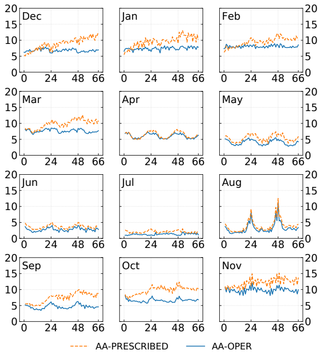
Figure 12. Monthly root mean square error (RMSE) of the ice surface temperature as a function of lead time for forecasts initialized at 00:00 UTC for AA-PREScribed and AA-OPER (snow-free SICE configuration). Monthly RMSEs are calculated using the MODIS ice surface temperature product and cover the time period from 1 December 2015 to 1 December 2016; x axis: forecast lead time from 00:00 UTC (h); y axis: RMSE of the ice surface temperature (°C).
