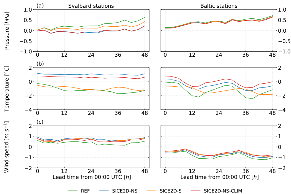
Figure 3. Mean error as a function of lead time for forecasts initialized at 00:00 UTC for experiments REF, SICE2D-NS, SICE2D-S, and SICE2D-NS-CLIM over the AROME Arctic domain for the period from 1 March to 30 April 2013. Left panels: for seven Svalbard stations (WMO nos. 01005, 01006, 01009, 01011, 01016, 01020, 01062). Right panels: for seven stations in Gulf of Bothnia (WMO nos. 02269, 02287, 02297, 02862, 02863, 02873, 02910). The mean error is calculated as the forecasted value minus observed value. (a) Mean sea level pressure; (b) 2 m temperature; (c) 10 m wind speed.
