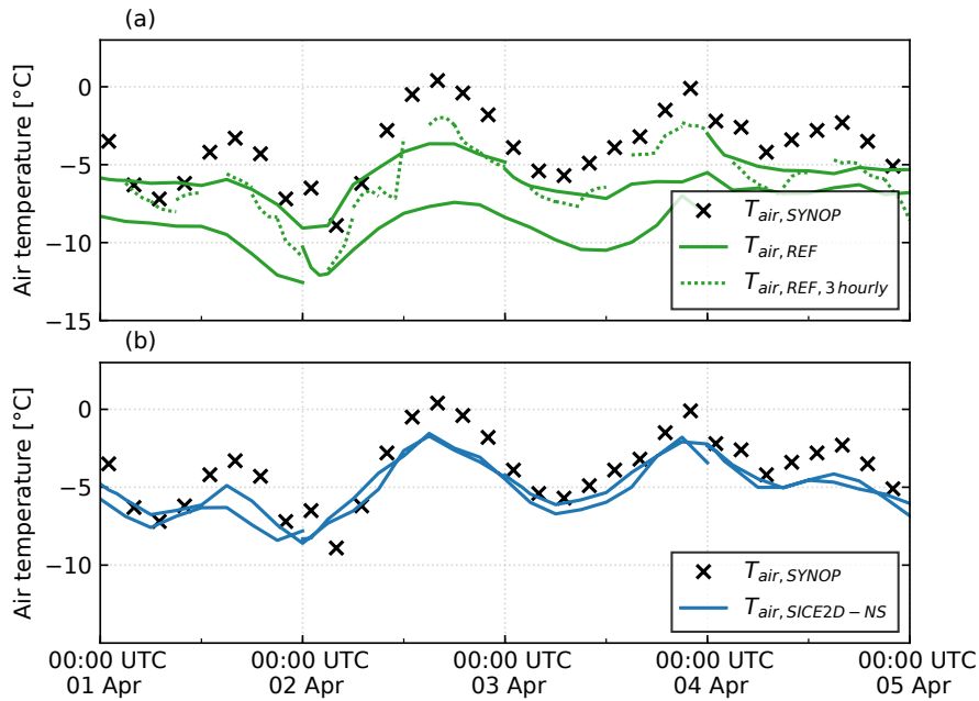
Figure 7. Evolution of the 2 m temperature for the Kemi I lighthouse station (WMO no. 02863; 65°25′ N, 24°08′ E) observed (black crosses) and simulated by the 48 h forecasts initialized at 00:00 UTC for experiments (a) REF and (b) SICE2D-NS. Also in (a), the simulated 2 m temperature values for the short 3 h forecasts initialized every 3 h (except 12:00 UTC, which is not shown) that are needed for the initialization of the long forecasts are shown (dotted lines).
