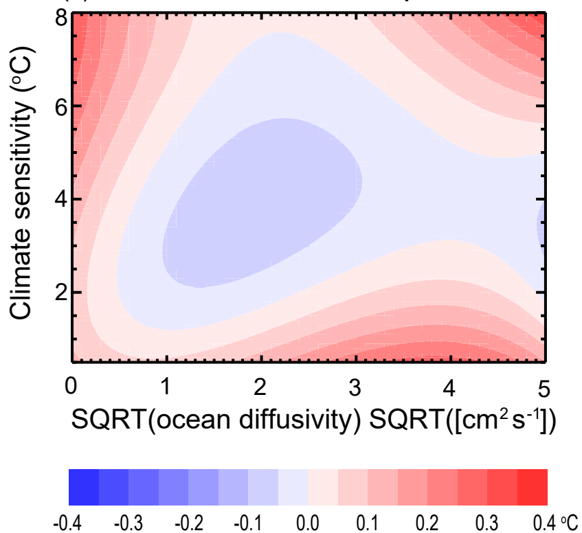
(c) transient climate response
