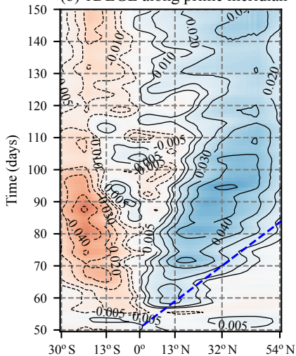
(b) IDEGL along prime meridian
