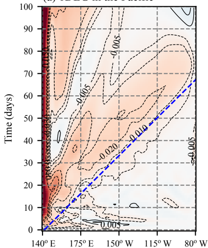
(a) IDEG in the Pacific
