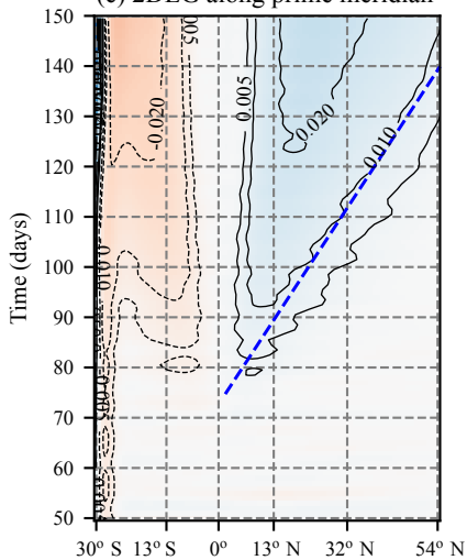
(c) 2DEG along prime meridian
